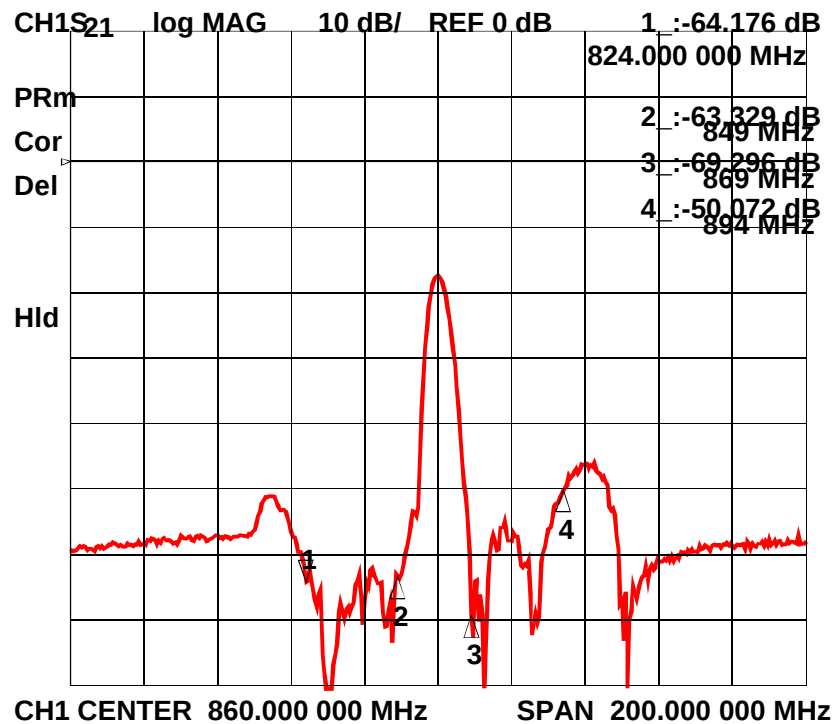
Figure 3-2 Electrical Characteristics
