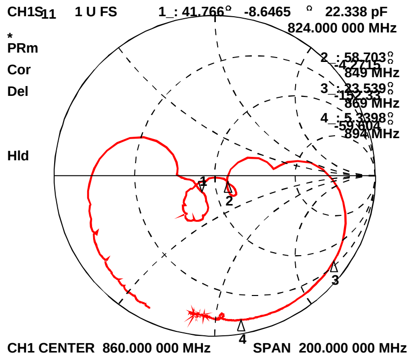
Figure 3-3 Electrical Characteristics
