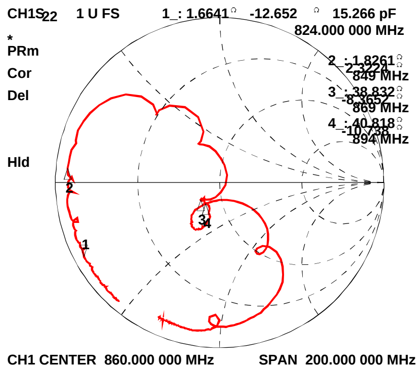
Figure 3-5 Electrical Characteristics
